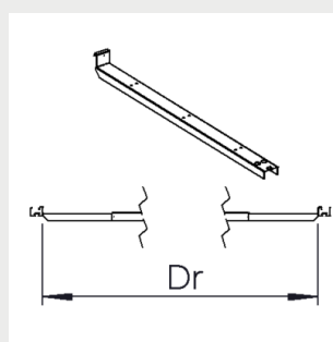
Omega/ALG2 railbracket (4)
